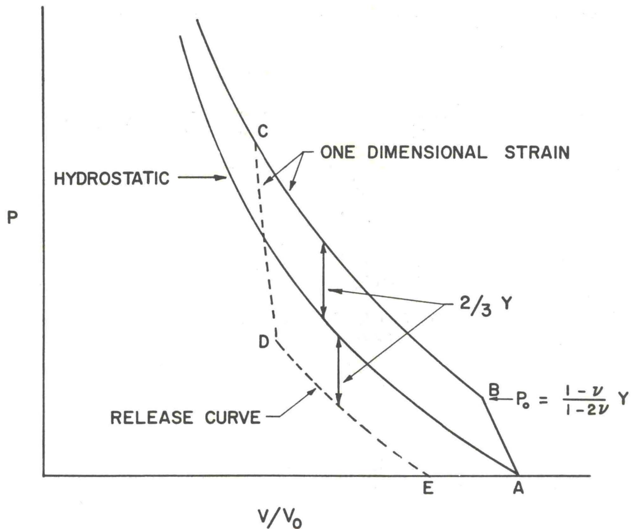
Figure 12. Stress-Volume Curves for One-Dimensional Strain Based on Elastic-Plastic Model. Relief of stress from a (shocked) state "C" follows path CDE. P_0 is Hugoniot elastic limit, Y is yield stress.
